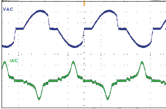
Trailing-Edge Dimmer
