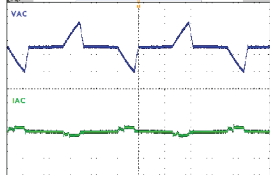
Trailing-Edge Dimmer
